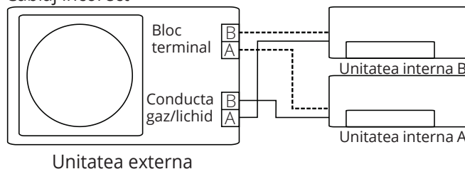
Cablaj incorect
