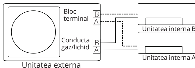
Cablaj incorect
