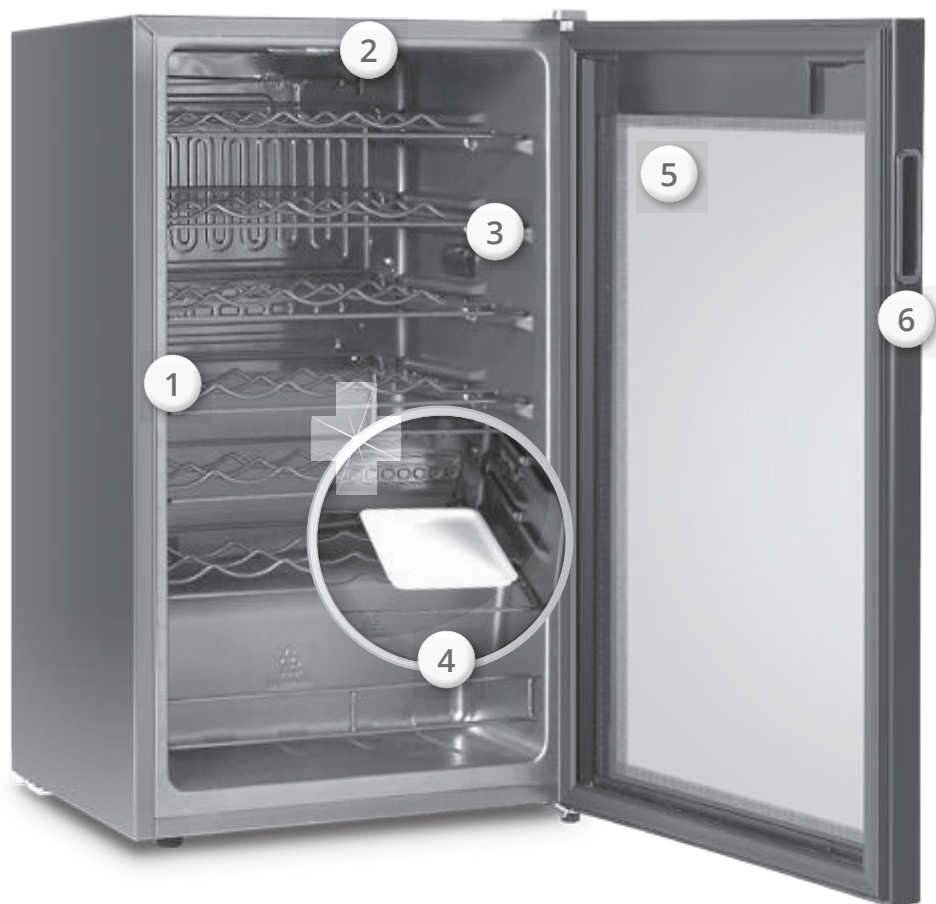
1. Wine Racks 2. Led Light 3. Dry filter 4. Water tray 5. UV glass door 6. Handle 7. Temperature Control Display 8. Adjustable Feet 9. Power Cord
